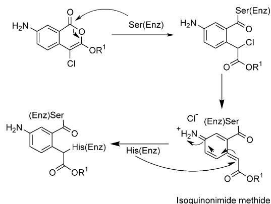
Scheme 4.
