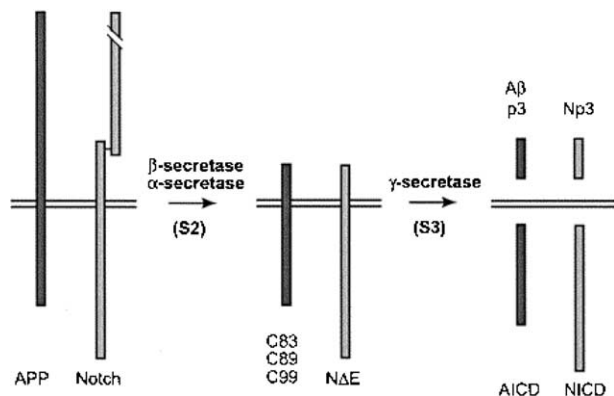
Scheme 1. APP and Notch secretase proteolysis, according to Wolfe et al. 14
