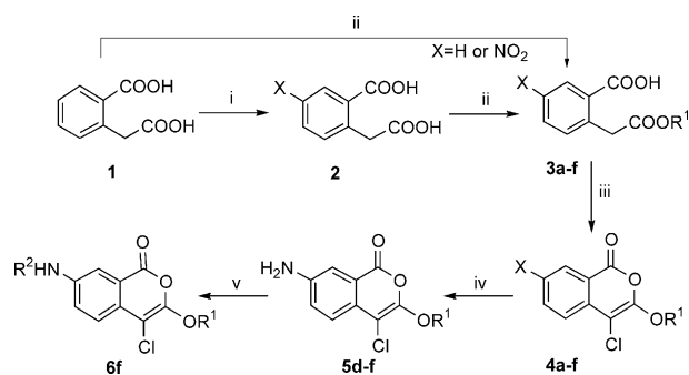
Scheme 2. (i) Fuming nitric acid, 2 h, rt; (ii) \text{R}'\text{OH} , [\text{H}_2\text{SO}_4] , heat; (iii) \text{PCl}_5 , toluene, reflux, 15 h; (iv) \text{H}_2/\text{Pd/C} , THF, rt; (v) adamantyl fluoroformate, TEA, THF, rt, 3 days.
